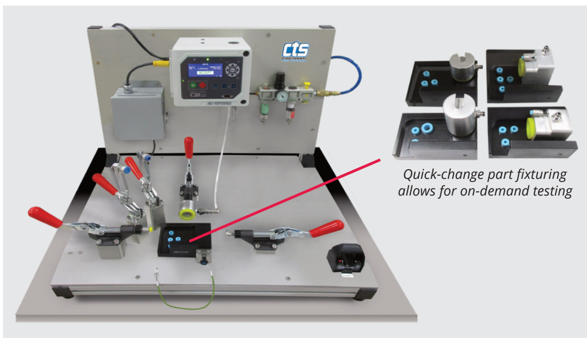
Custom benchtop leak test system utilizing the C20 pressure decay instrument with interchangeable fixtures to test a variety of parts
